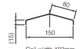
Coil width 183mm
