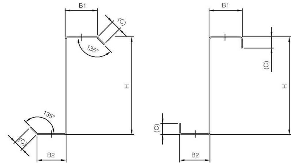
Z型檩条规格 Sizes of Z-shape purlins
