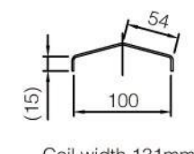
Coil width 131mm
