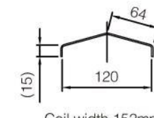
Coil width 152mm
